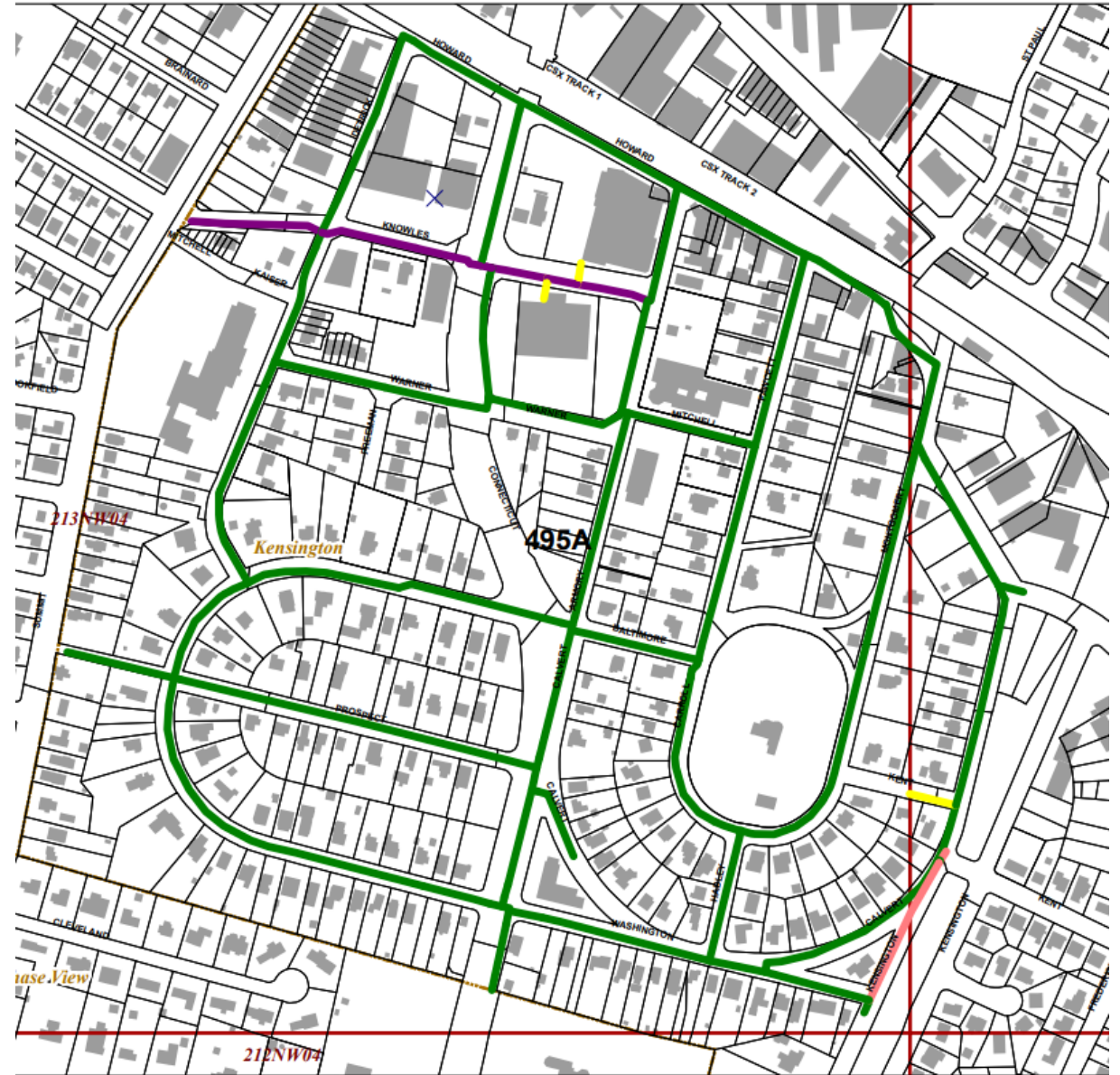
WARNER CIRCLE WATERMAIN REPLACEMENT - PROPOSED CONDITIONS EVALUATION MAP 213NW03 & 213NW04
