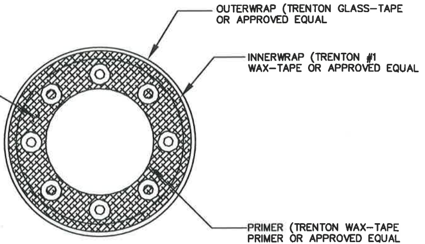
SECTION VIEW "B-B"
