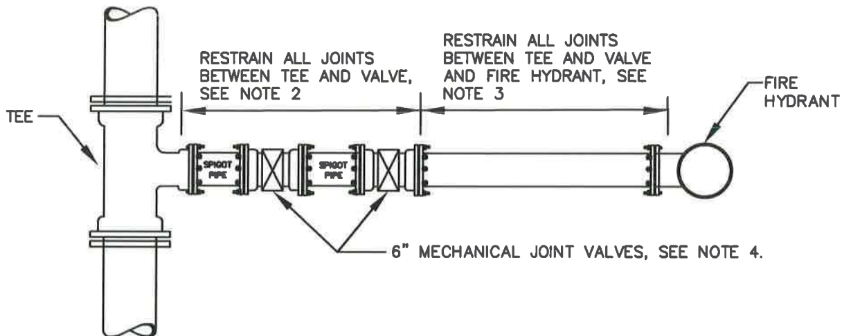
PLAN - 36" AND LARGER MAINS
