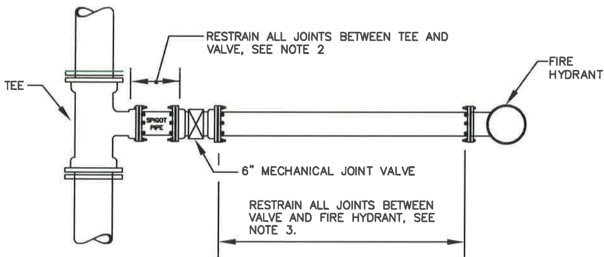
PLAN - 14" TO 30" MAINS
