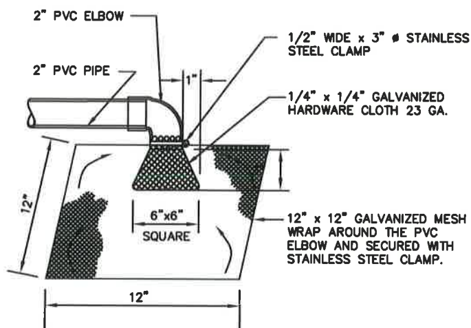
BIRD SCREEN DETAIL
