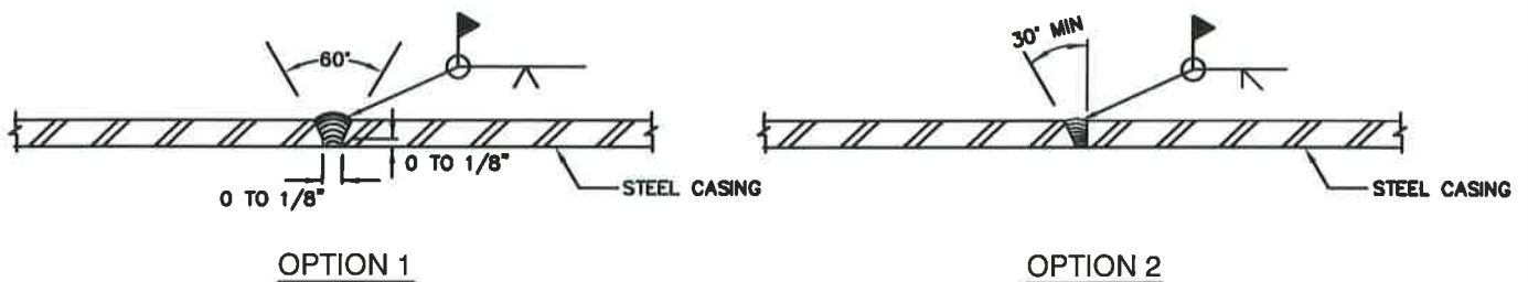
STEEL CASING WELD DETAIL (TYP.)
