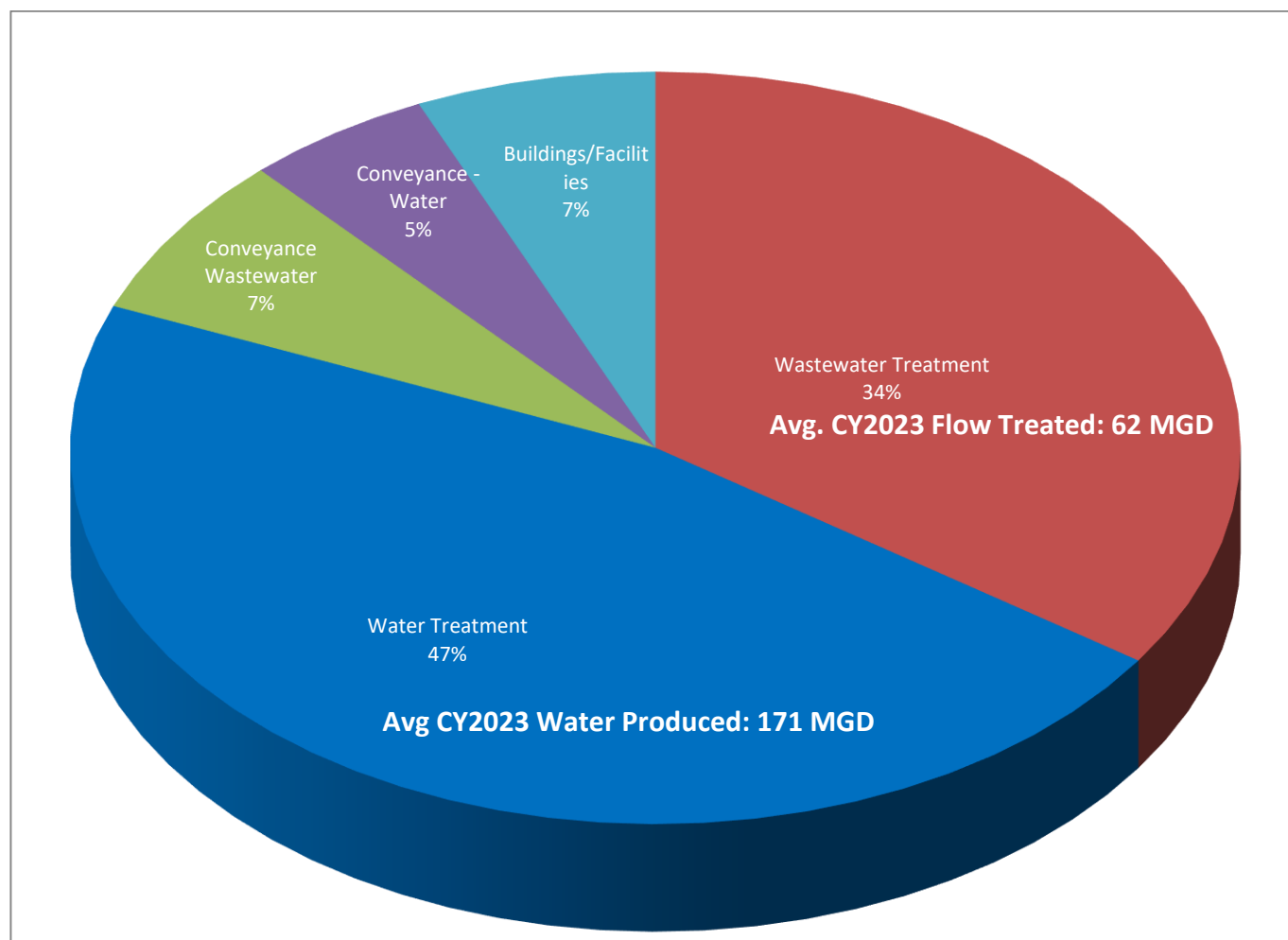
FIGURE 2-2 Comparison of 2022 Electricity Usage by Category
