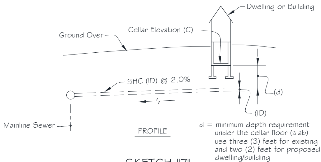
SKETCH "Z" Determining SHC Invert Elevation at Mainline Sewer
