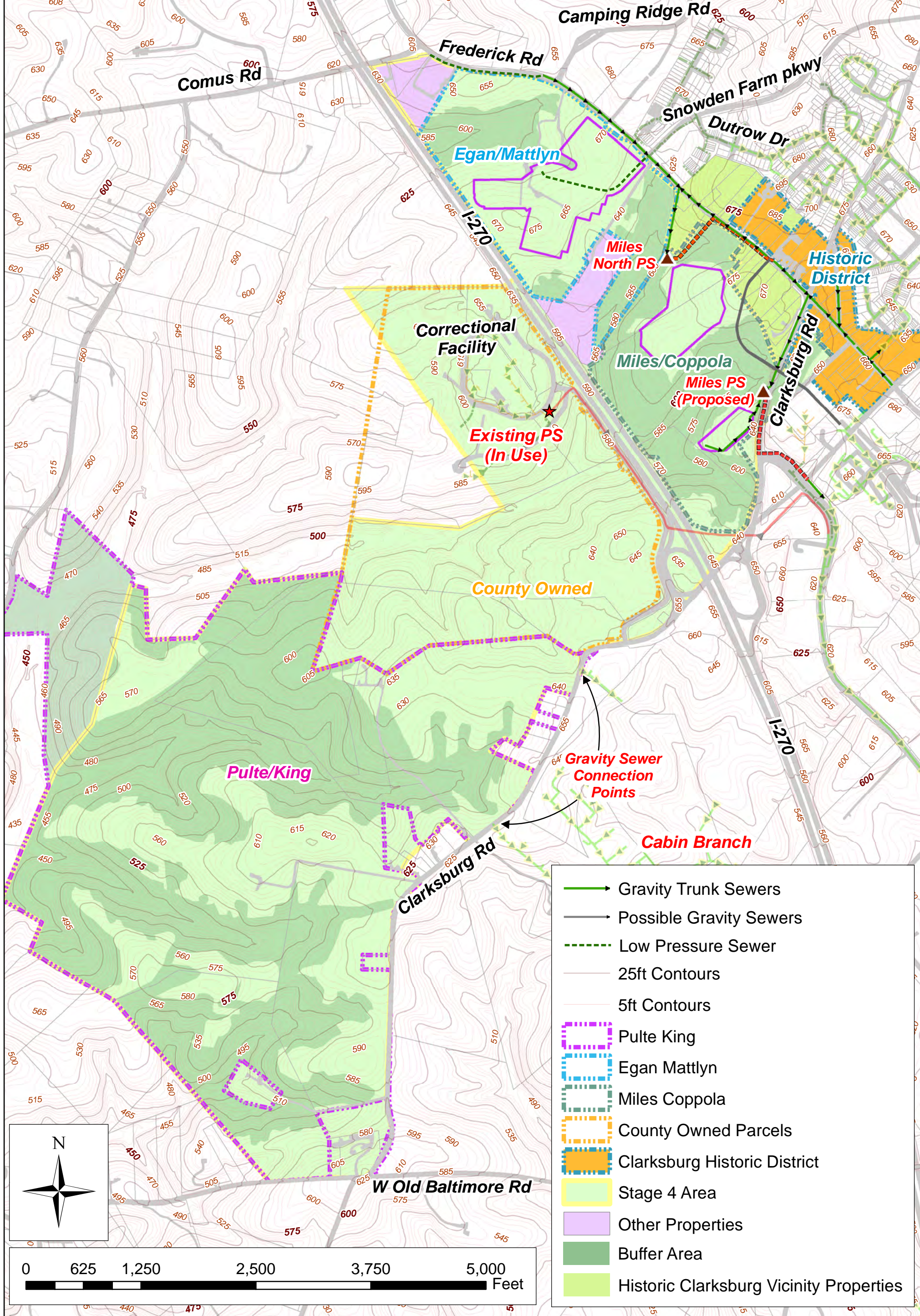
Figure 3-7 Alternative 7 - Gravity + 3 Pump Stations and Grinder Pump Systems
